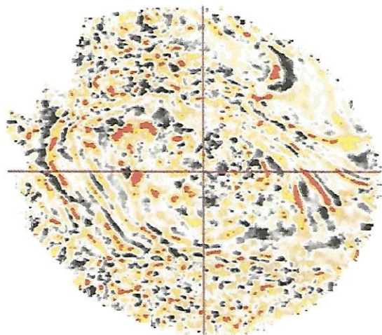
Figure 7a PSTM time slice after conventional processing and binning.
